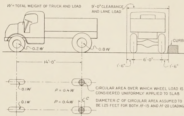
FIGURE 1.—DIAGRAM OF TRUCK LOADING.
